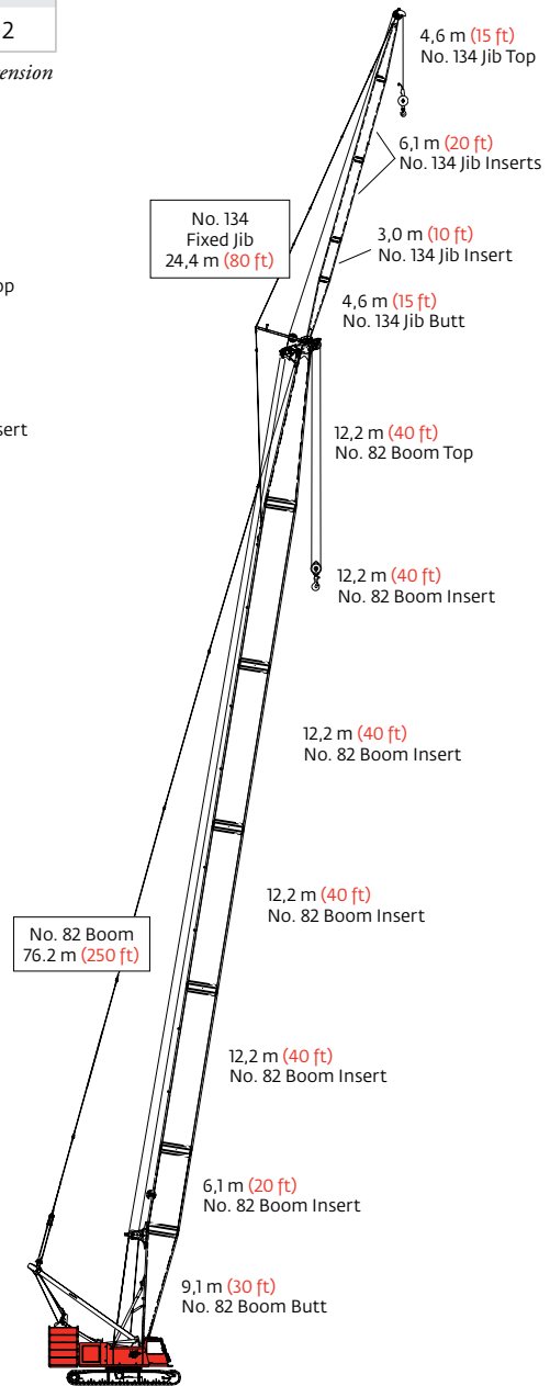
Model 999 Series 3 No. 134 Fixed Jib on No. 82 or 22EL Boom 100,6 m (330 ft)
